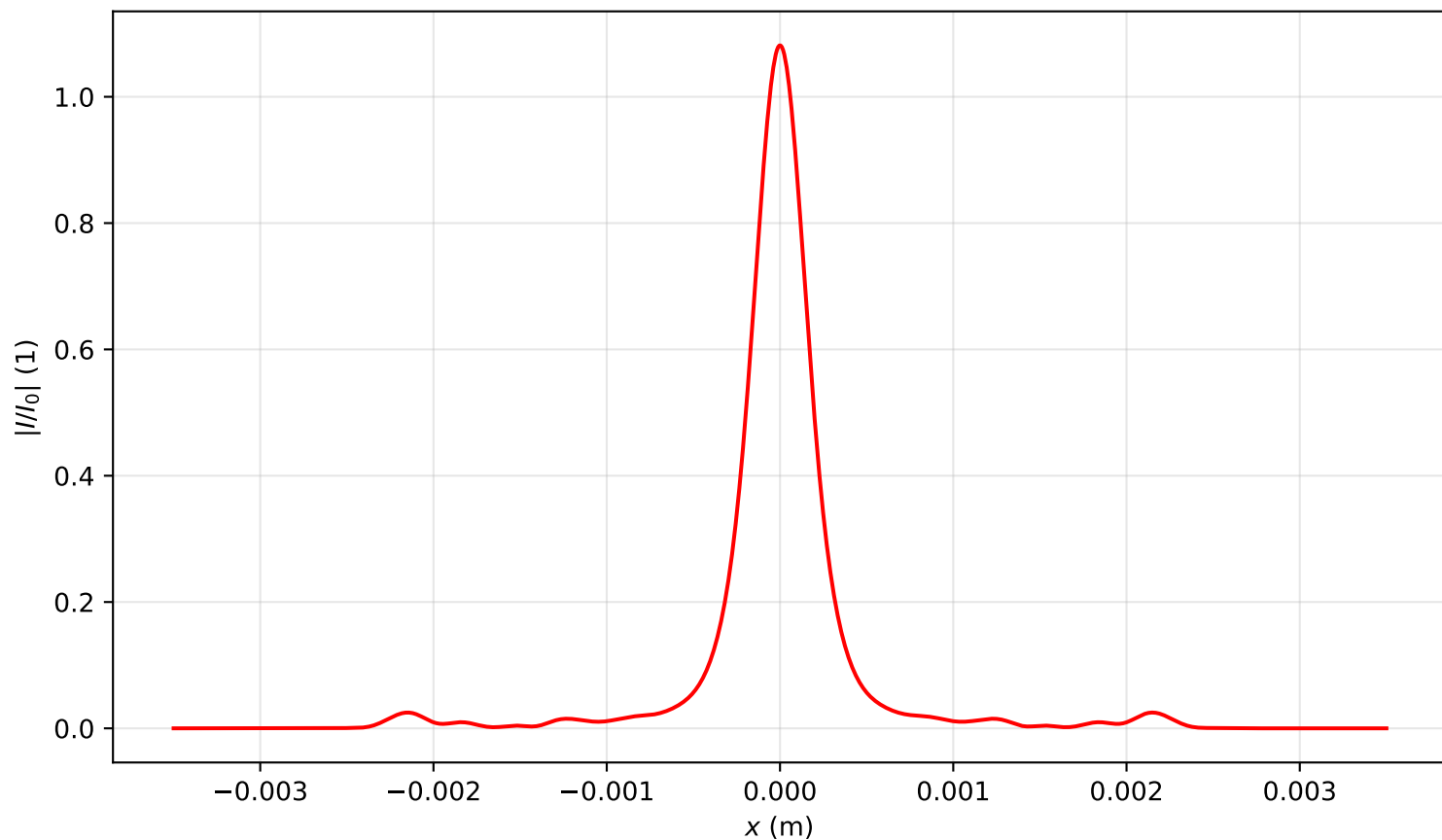
Intensity profile I(x, y = 0, z = 3.821)/I_0 , \text{Pin}=3.5\text{Pcr} , artificial time
